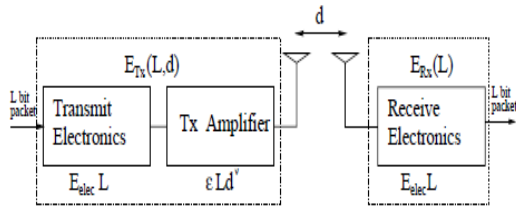
Fig.2. Radio Model
